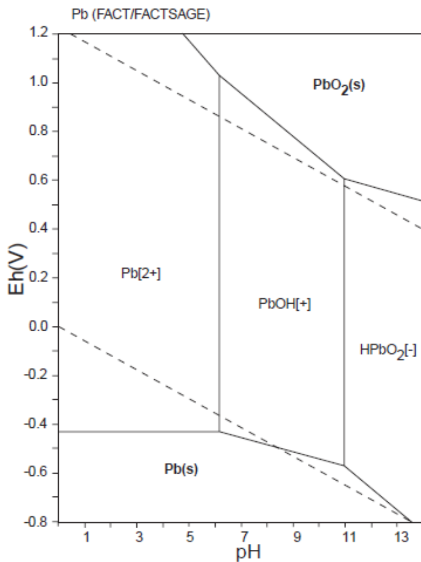
Figure 90: Eh-pH diagrams of the system Pb-O-H (1). \Sigma \text{Pb} = 10^{-10} , 298.15K, 10^5 Pa.
