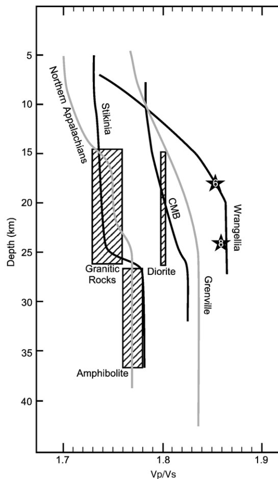
Fig. 5. The seismic property V_p/V_s of three intervals along the section shown in Fig. 3, compared with V_p/V_s from the Grenville province [25], the northern Appalachians [25], and V_p/V_s for gabbro (stars labeled 6 and 8, for 6 and 8 kbar [24]). V_p/V_s of CMB and Wrangellia from [7], that of Stikinia from [11] and [44]. Shows striking difference of crustal lithology between the three ACCRETE panels, and similarities to the other crustal sections. The approximate uncertainty for the three ACCRETE crustal sections and for the Grenville and Appalachian sections is \pm 0.02 [7,25]; that for gabbro is \pm 0.03 [24]. V_p/V_s for diorite and granitic rocks were taken from rock measurements [7] and the values for amphibolite are based on data in [24] and [25].
