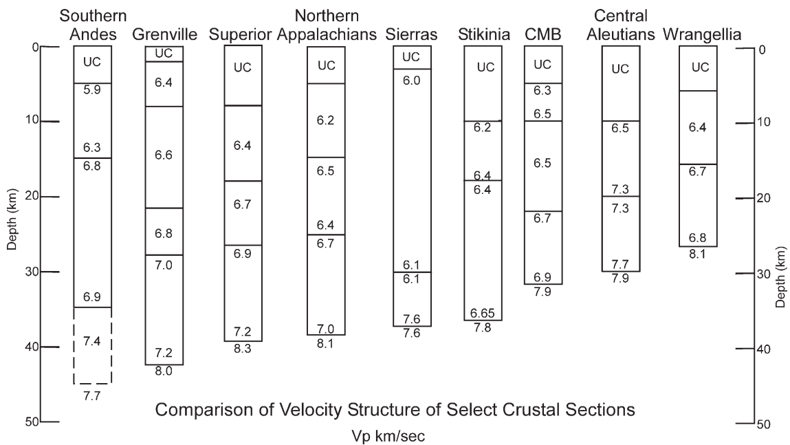
Fig. 4. Comparison of compressional wave velocities ( V_p , km/s) and thickness for several crustal sections, arranged by thickness, with those for the three crustal panels of Fig. 3: Wrangellia, the CMB, and Stikinia. V_p for upper crust (UC) not shown. Values of V_p are shown above and below depth markers, or between them if variation is minimal. All data are from controlled source seismic refraction experiments except those for below 35 km of the southern Andes, which are based on a receiver function study [40]. Sources: southern Andes [40], Grenville province [25], Superior province [41], northern Appalachians [25], southern Sierra Nevada batholith [42], Stikinia [11], Coast Mountains batholith [8], central Aleutians [43], Wrangellia [39].
