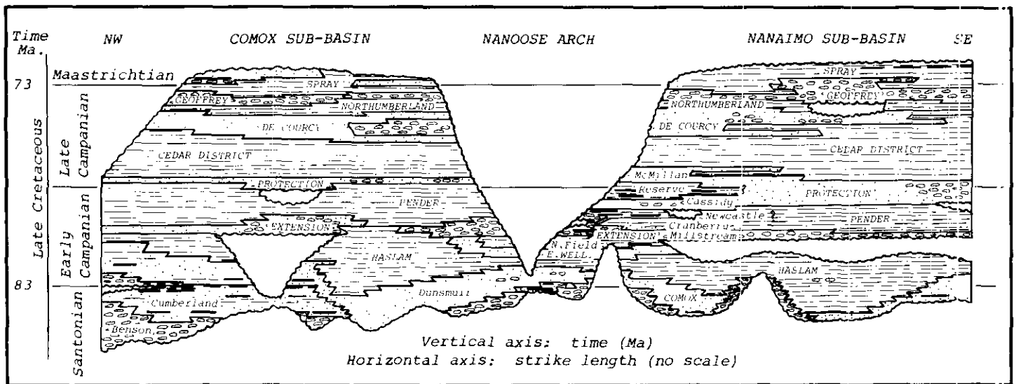
Figure 4-3-2. Stratigraphic relationships of the Nanaimo Group. Refer to Table 4-3-1 for legend.
