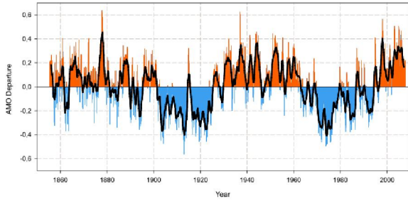
Monthly values for the AMO index, 1856–2008
