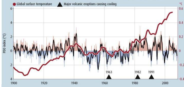
The Pacific Decadal Oscillation index – the relative mean surface temperature of the Pacific north of 20° latitude (adjusted to exclude the long-term warming trend). Low values are linked to lower global surface temperatures
